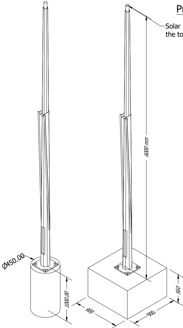
Configuration 1 SCALE 1/30 Configuration 2 SCALE 1 / 30
