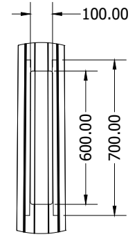
DETAIL B SCALE 0.06 : 1
