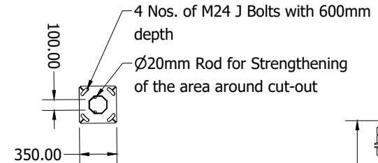
SECTION G-G SCALE 1 / 35
