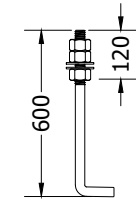
DETAIL G.1 SCALE 1 / 35
