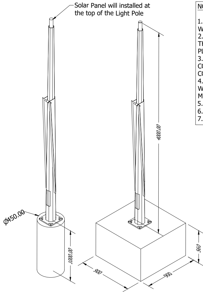
Configuration 1 SCALE 1/25
